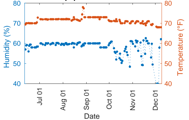
Equipment Room
